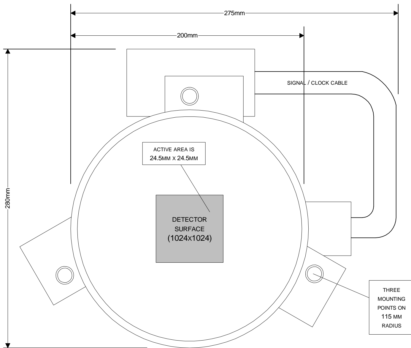
FRONT VIEW OF STANDARD CCD CRYOSTAT
