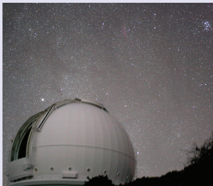
Left: Awarded photograph of NGC 2246, the Rosette Nebula by Mischa Schirmer. The image was obtained through an H \alpha filter on a 2x2 mosaic of 21 images totalising an exposure time of 3 hours and 30 minutes. Right: Picture of the WHT taken by Nik Szymanek with a digital camera.
