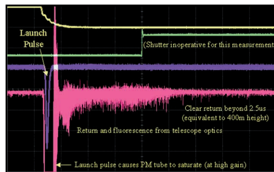
Figure 4. Fluorescence measurement.
