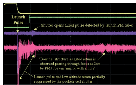
Figure 5. Range-gated return.
