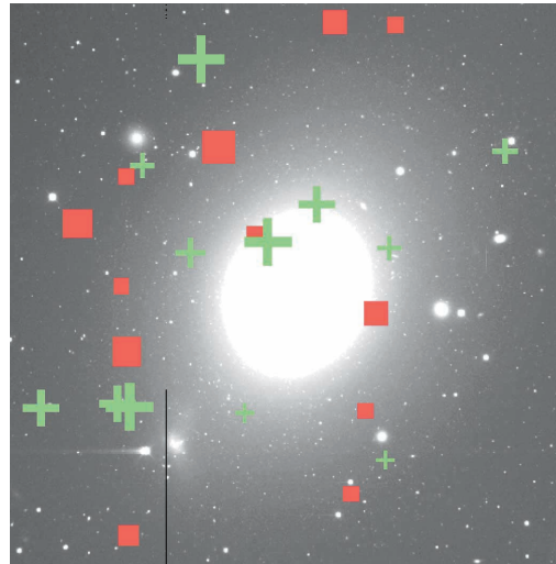
Figure 1. Planetary nebula velocities in NGC 4472, relative to a systemic velocity of 977 km/s. Green crosses represent negative velocities, and red boxes represent positive velocities, where the symbol sizes are proportional to the velocities. North is at the top and east at the left. The underlying image is from X. Hui, with a field-of-view of 16' \times 16' .
