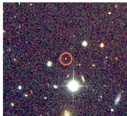
Figure 4. A colour composite image of wfsj2245+0024 made from the INT WFS 600 second exposures in g' , r' and i' . The object was identified as a candidate high redshift ( z>5 ) quasar by the red colour.
