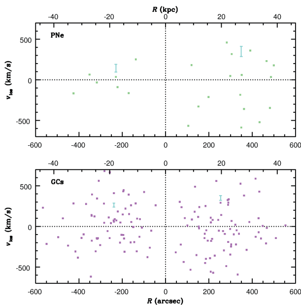
Figure 2. Line-of-sight velocities of planetary nebulae (top) and globular clusters (bottom) as a function of radius, relative to the central velocity of NGC 4472. Objects with a positive radius lie on the northeast side of the galaxy's major axis, and those with a negative radius on the southwest side. The overall velocity dispersion on either side is marked with error bars.
