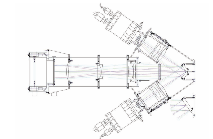
Figure 5. Sketch showing the optical arrangement of the Planetary Nebula Spectrograph. On the right-hand side, a pair of diffraction gratings can be seen to split the light beam into two identical spectrograph arms, each with a different dispersion direction.
