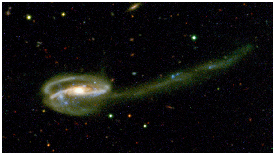
Figure 3. The false colour image ( u' , g' , i' filters) of galaxy UGC 10214, thanks to Simon Hodgkin at Cambridge Astronomical Survey Unit (CASU).
