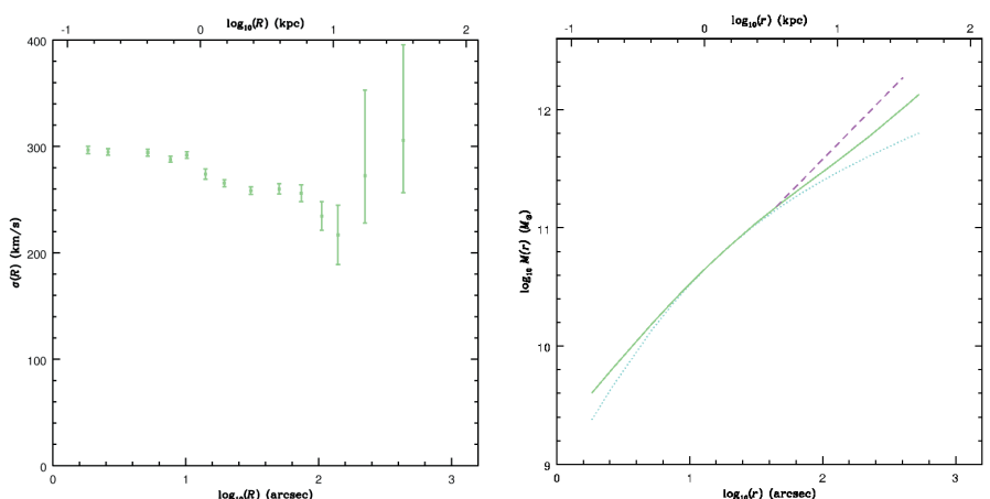
Figure 3 (left). Stellar projected velocity dispersion as a function of radius for NGC 4472, with 1-\sigma error bars. The first 12 points come from the integrated light spectroscopy of Fisher, Illingworth, & Franx (1995). The last 2 points represent our planetary nebulae data. Figure 4 (right). Enclosed mass as a function of radius for NGC 4472. The solid line shows the results derived from the stellar kinematics (integrated light + planetary nebulae), assuming an isotropic distribution function. The dashed line shows the results from the globular cluster kinematics, also assuming isotropy (Zepf et al., 2000). The dotted line shows a constant mass-to-light ratio model.
