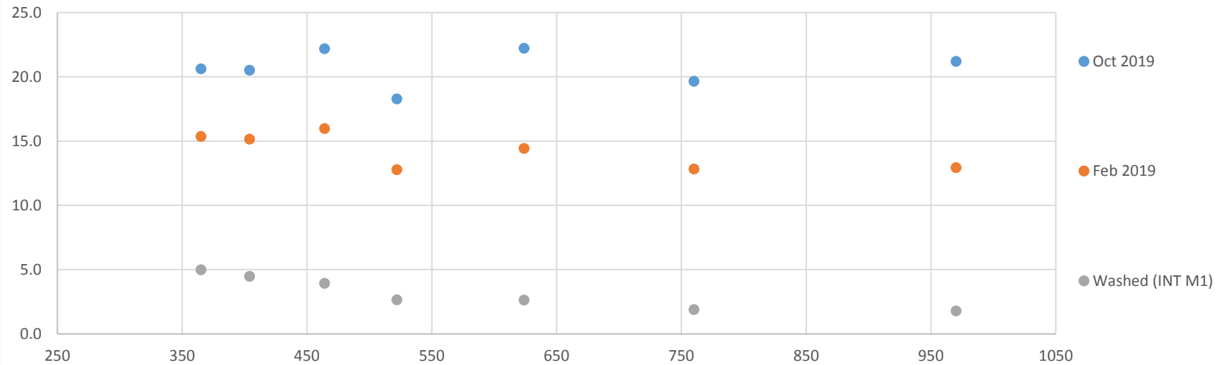
Scattering of M1, Oct 2019 and gain from washing
