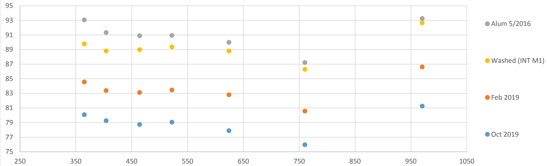
Reflectivity of M1, Oct 2019 and gain from washing
