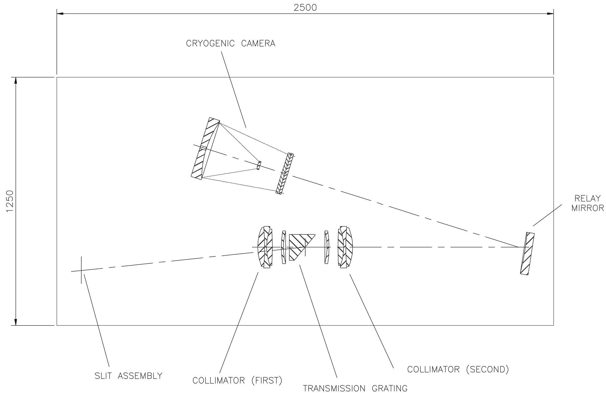
WYFFOS—OPTICAL ARRANGEMENT — TRANSMISSION GRATING
