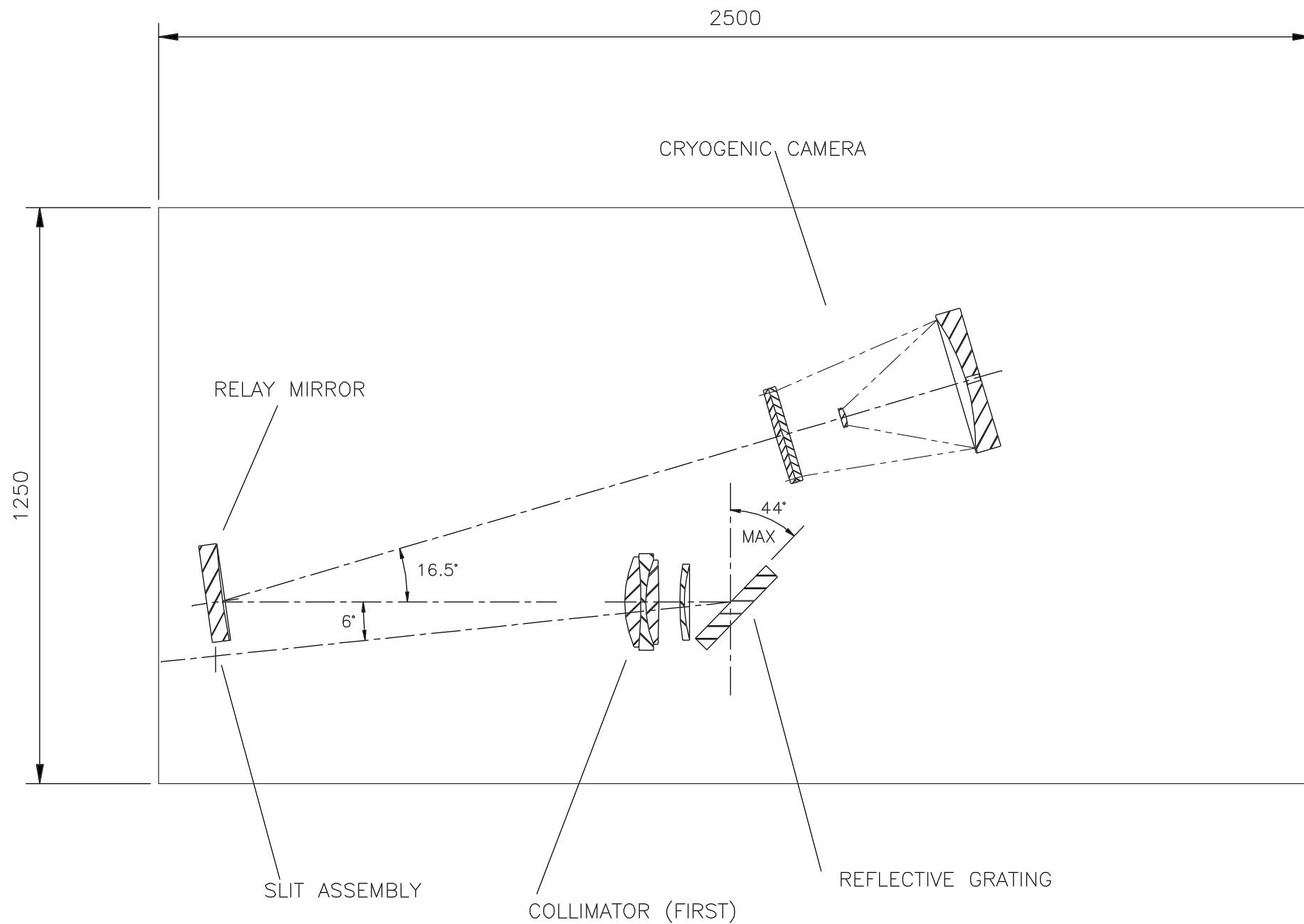
WYFFOS—OPTICAL ARRANGEMENT — REFLECTION GRATING
