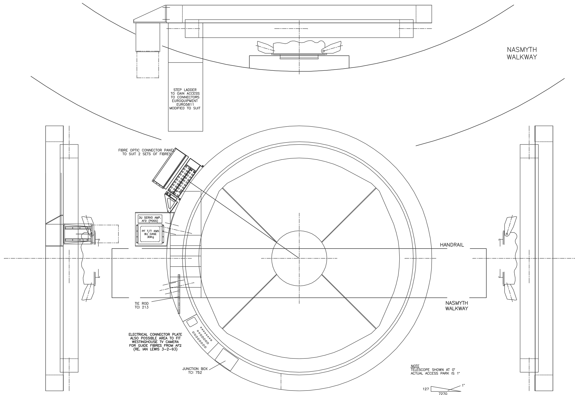
4.2m WHT TOP END SHOWING PROPOSED LAYOUT OF EQUIPMENT REQUIRED TO BE FIXED TO THE TOP RING
