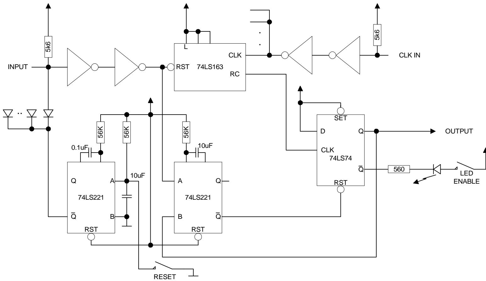
TYPICAL DEBOUNCE CIRCUIT. 1 OF 7
