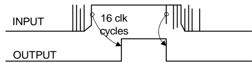
WAVEFORMS
