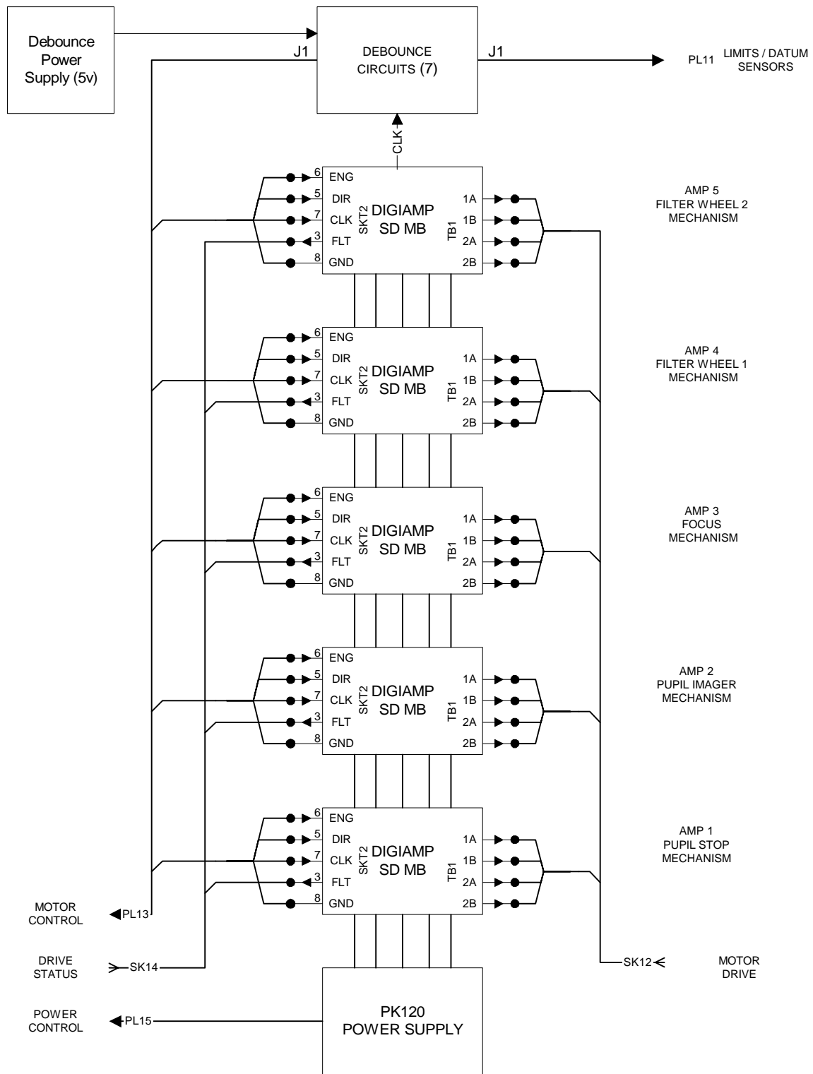
INGRID MECHANISM AMPLIFIER CHASSIS
