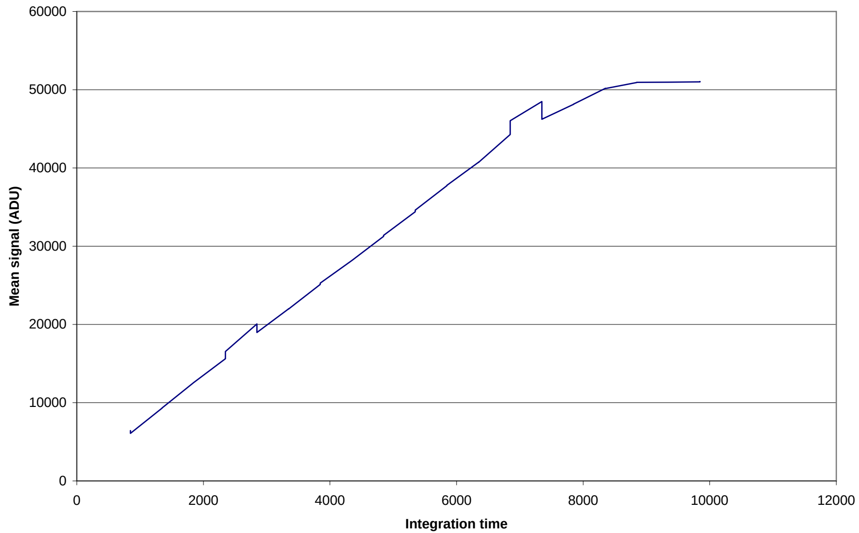
Photon transfer Vrst 0.95
