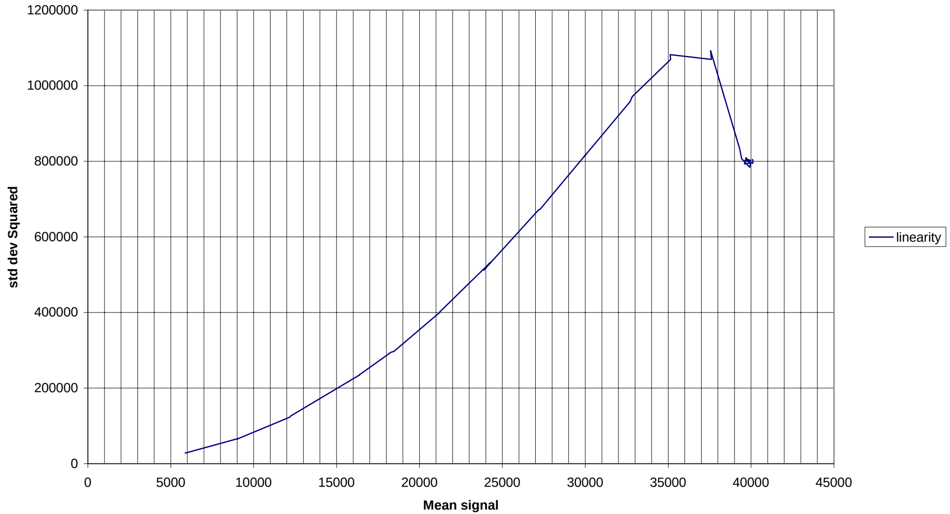
linearity Vrst 0.75
