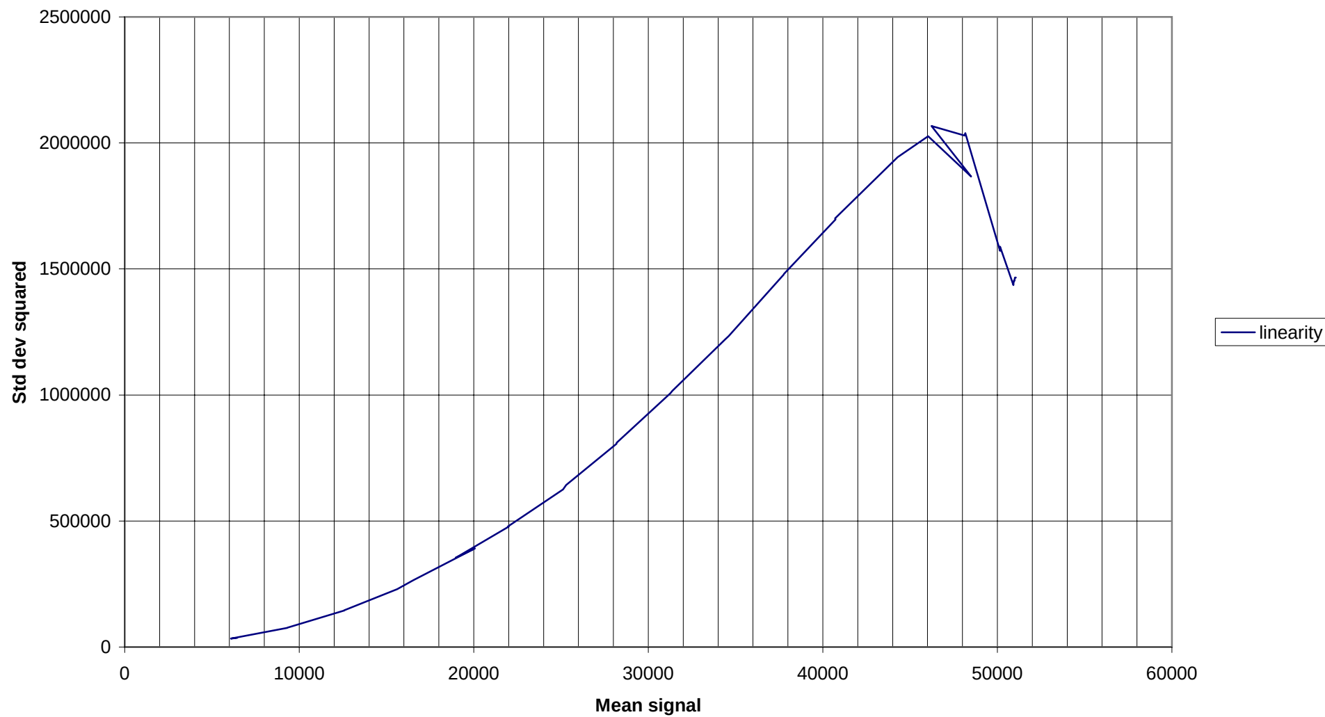
linearity Vrst 0.95
