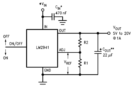
5V to 20V Adjustable Regulator
