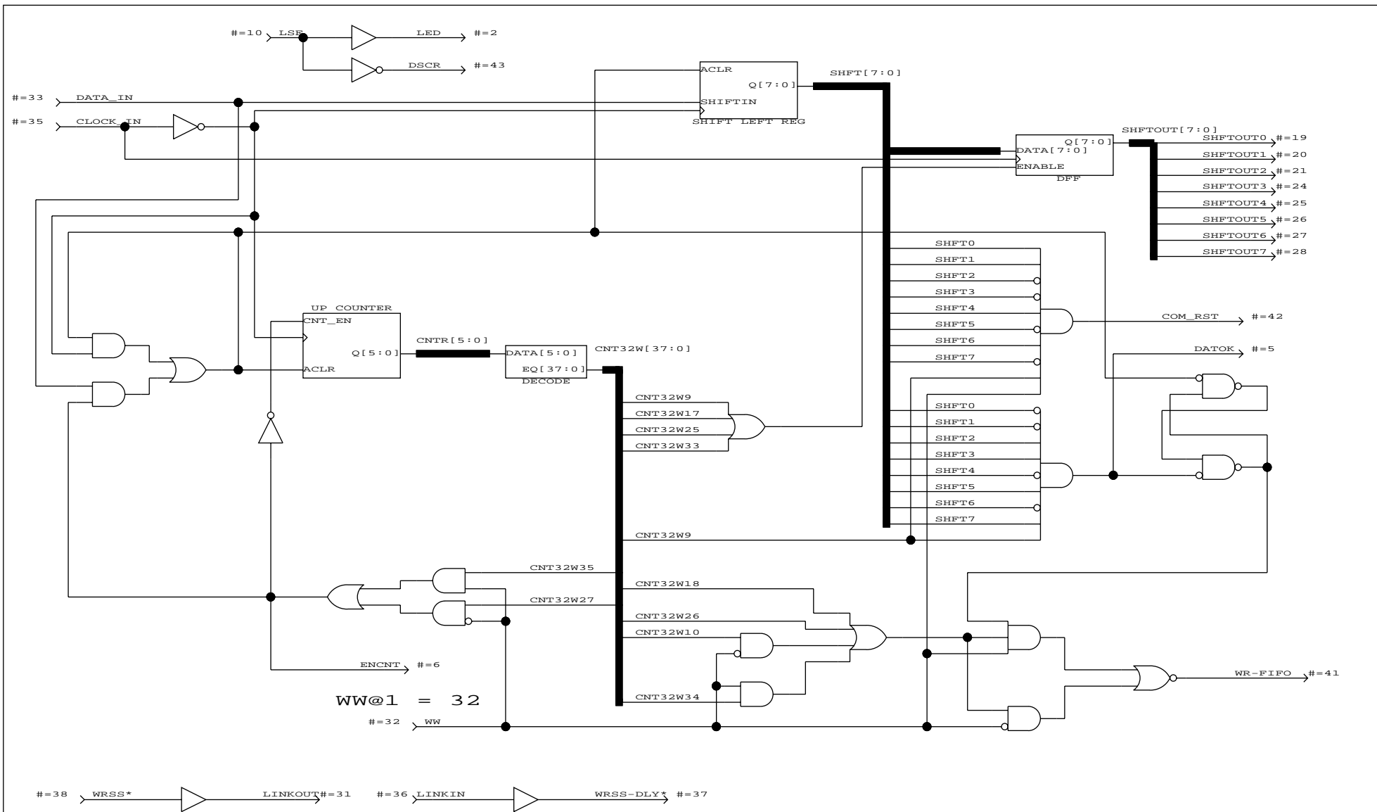
TIMING BOARD FIBER OPTIC INTERFACE U2 REV 4B 10/4/97
