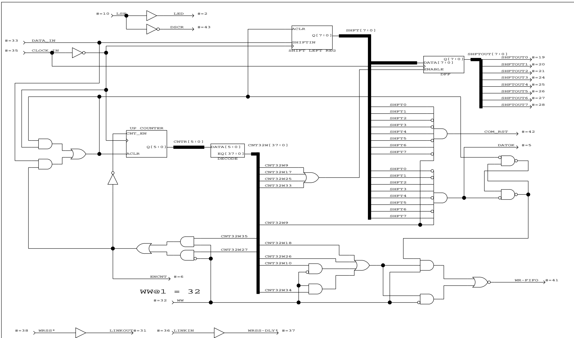
TIMING BOARD FIBER OPTIC INTERFACE U2 REV 4B 4/9/97
