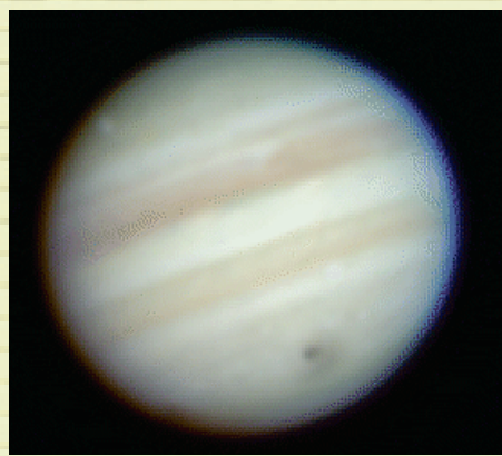
In July 1994 the individual fragments of Comet Shoemaker-Levy 9 impacted onto the planet Jupiter. Images obtained from the 1m Jacobus Kapteyn Telescope clearly showed the ejecta plume of debris rising over the planet's limb from the impact site of fragment L. At the same time the 2.5m Isaac Newton Telescope was used to observe spectroscopic emission from the vaporised comet, revealing some of its constituent elements. Finally, continued imaging showed clearly the effects on the Jovian atmosphere, as in the image above of the impact site of fragment G.
