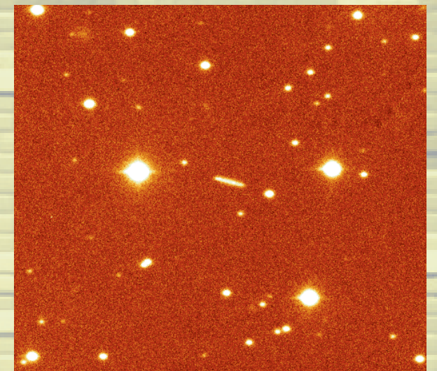
Asteroid 3634 Iwan (the straight line in the middle). Image obtained on the night of 30/31 August 1995. ING telescopes have also observed and discovered the most distant Kuiper Belt objects. This is a 2.8x2.8 arcmin image obtained using the 1.0m Jacobus Kapteyn Telescope.
