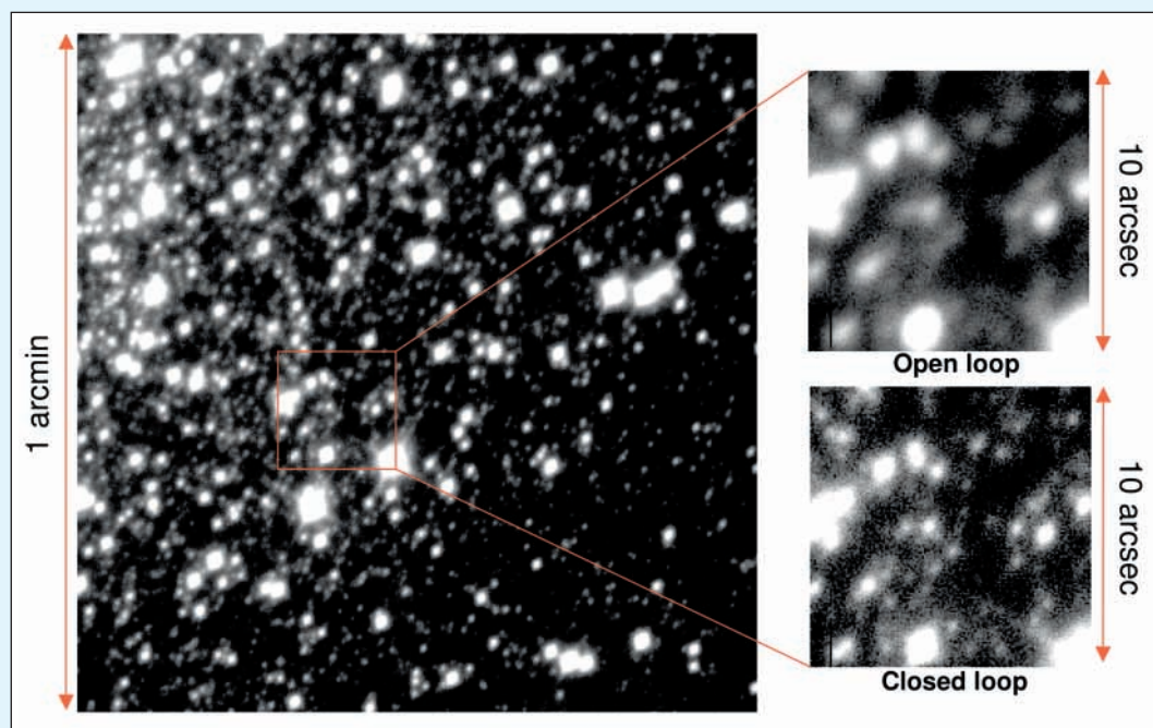
This H-alpha image (top) of globular cluster M13 was taken with the WHT's adaptive-optics system NAOMI. The FWHM has been improved from 0.8 arcsec (natural seeing) to 0.4 arcsec, allowing many faint stars to be resolved. The image was taken during September 2001 tests of NAOMI's performance at optical wavelengths, and provides a realistic outlook of the AO potential at the William Herschel Telescope. Given that the median natural seeing on La Palma is about 0.7 arcsec, an image quality of \sim 0.3 arcsec in the R and I bands should be achieved regularly.
