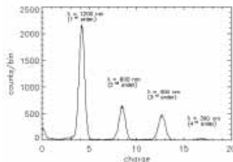
Figure 3. Wide band response of STJ.
