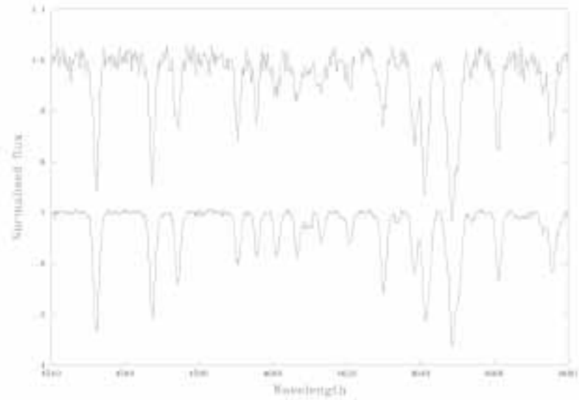
Figure 2. This figure compares spectra of the M31 and Galactic B1 Ia supergiants OB78-159 (top) and HD194279 (bottom). The spectral range covered contains the Si III triplet at 4553/4567/4574\text{\AA} , and a number of O II and N II lines between 4590 and 4680\text{\AA} . The M31 spectrum is a 1 hour exposure obtained with ISIS on the WHT at a resolution of 5000 in half-arcsecond seeing, the star has a visual magnitude of 17.97 . The difference in the line strength ratios of O II 4590/4596\text{\AA} and the N II lines at 4601/4607 for example, is due to a slight temperature difference, OB78-159 being the hotter star. The detailed model atmosphere analysis of OB78-159 is underway, however we can already see that the metal line spectrum is consistent with a composition similar to supergiants in the solar neighbourhood.
