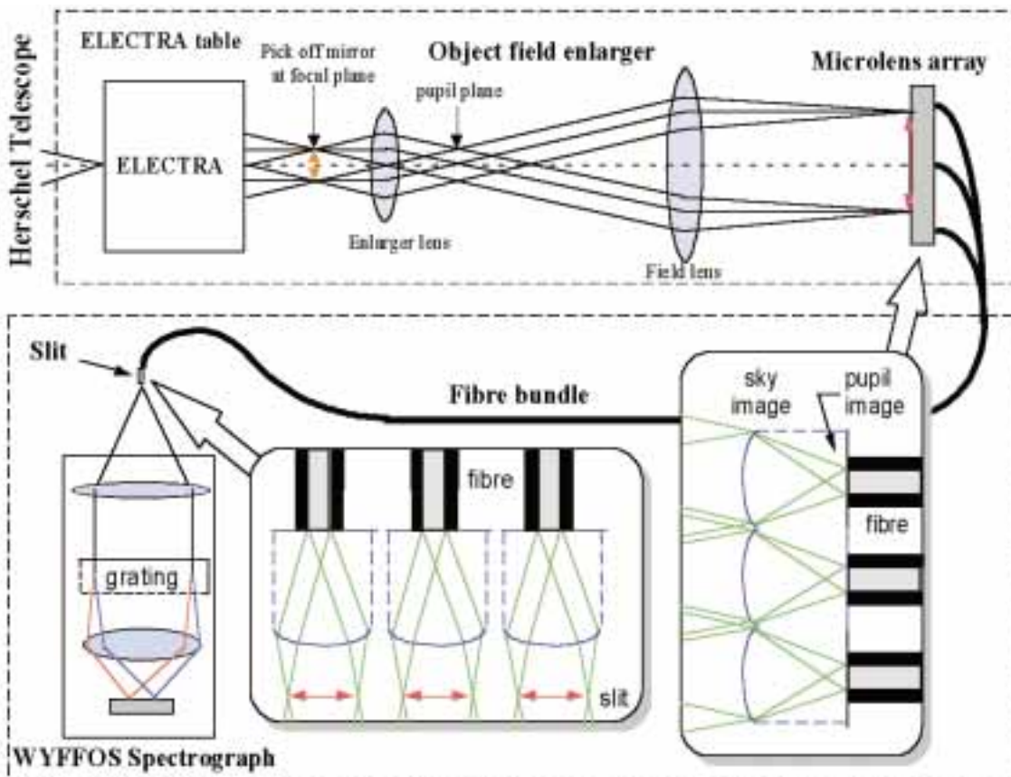
Figure 5. Principles of Operation of TEIFU.
