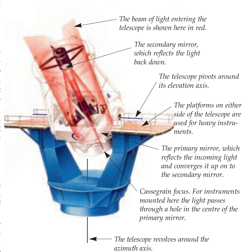
Above: Diagram of the WHT, showing the light path for the Cassegrain focus.
