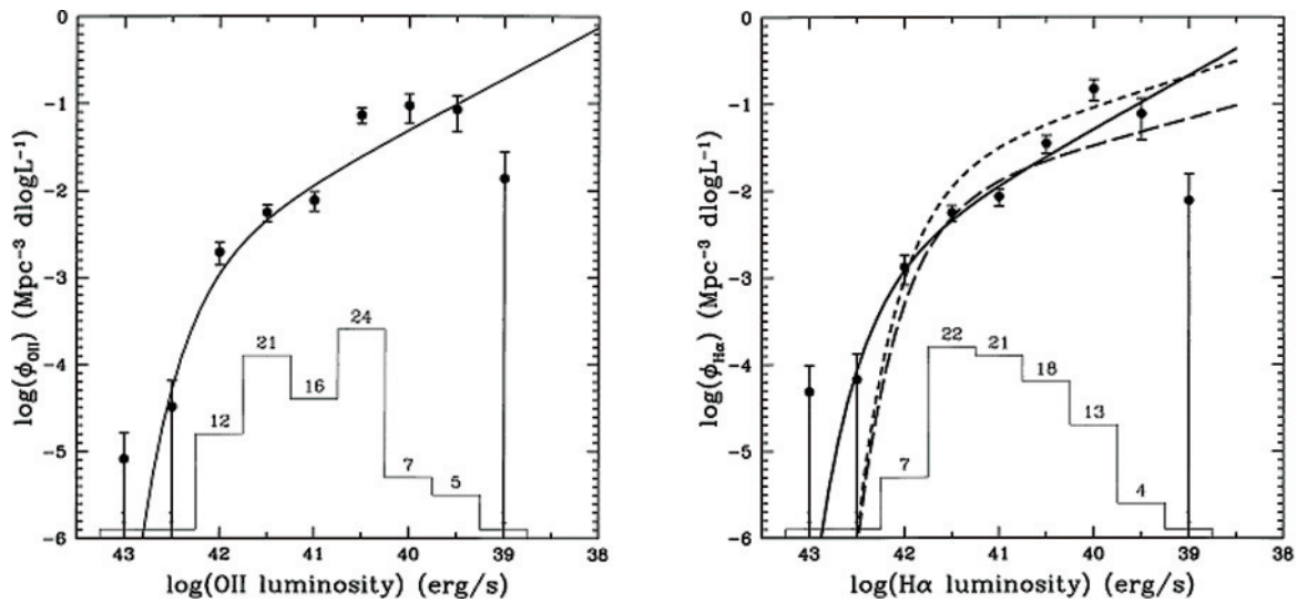
Figure 10. Left: The dust-corrected [O II] luminosity function derived from the AF2/WYFFOS sample (dots). The best fit is shown by the solid line. Right: The dust-corrected H\alpha luminosity function. The best fit is shown by the solid line. The short-dashed line is the H\alpha luminosity function derived by Tresse & Maddox, 1998 ( ApJ , 312, 691) in a similar redshift range, while the long-dashed line shows the z=0 estimate of Gallego et al., 1995 ( ApJ , 312, L1).
