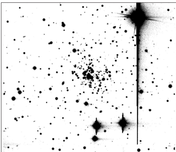
Central 4.3' x 4.3' image of Palomar 1, taken with the I filter and an exposure time of 600s.
