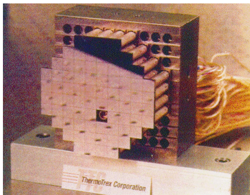
ELECTRA has a deformable mirror consisting of 76 individual segments. Each of the segments is driven by three (hysteresis corrected) piezoactuators, hence giving it 228-degrees-of-freedom. Hysteresis correction is maintained through strain gages on the piezos.
