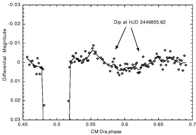
Planetary transit event candidate as observed at the JKT. The lightcurve is plotted against the phase of CM Dra. The data are shown as squares; the line indicates a smoothing fit to the data.
