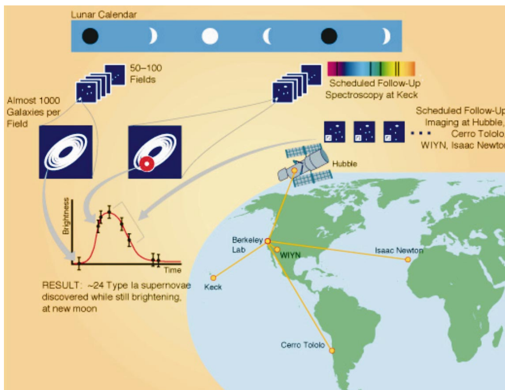
The observing strategy allows the team to find sets of high-redshift supernovae on the rising part of their light curves and guarantees the date of discovery, thus allowing follow-up photometry and spectroscopy of the transient supernovae to be scheduled. The supernova light curves are then followed with scheduled R-, I- and some B-band photometry at the INT and other telescopes.
