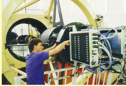
The INT Wide Field Camera (WFC) consists of a 4 chip mosaic assembly. A fifth CCD, a Lesser thinned Loral device, is co-mounted with the science array in the cryostat to provide autoguiding functions (see picture on the left). The picture in the middle corresponds to the first commissioning on the telescope in May 1997. Finally, the picture on the right is a true-colour image of M51 galaxy using BVR imaging on the WFC.
