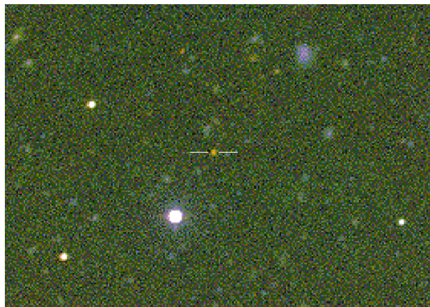
B and R image of GB1428+4217 (the very red object in the center). GB1428+4217 is the third most distant quasar and the highest redshift radio and X-ray source currently known. This picture was taken using the Prime Focus camera at the INT.
