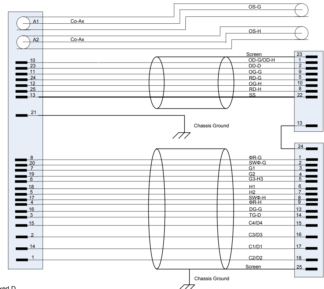
Front Panel Mixed D 25 power / 2 signal Connector A
