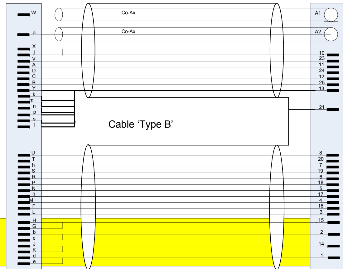
62GB-56T20-41 Connector B
