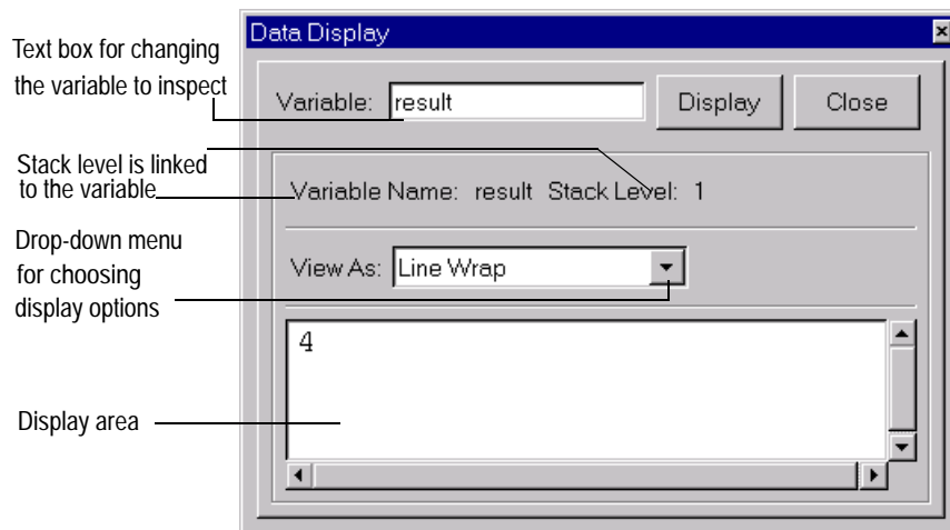
Figure 16 The Data Display Window
