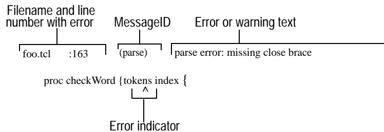
Figure 21 Anatomy of a TclPro Checker Message
