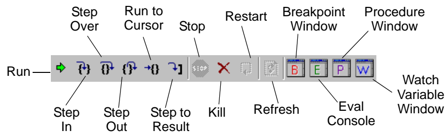
Figure 2 TclPro Debugger Tool Bar
