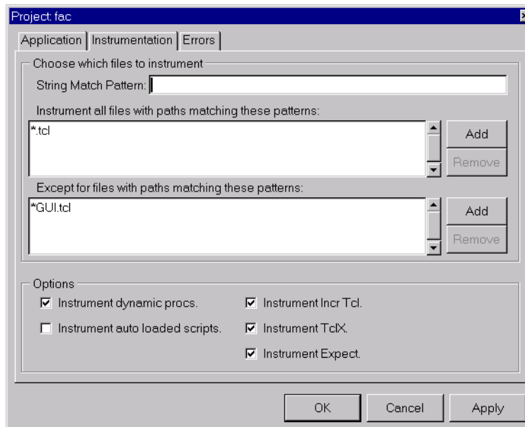
Figure 10 The Project Instrumentation Settings Tab
