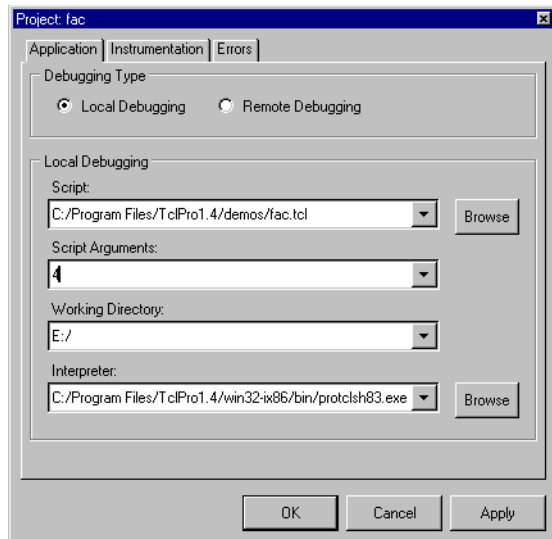
Figure 8 The Project Application Settings Tab, Local Debugging
