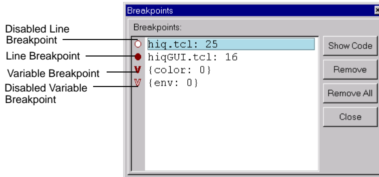
Figure 13 The Breakpoints Window
