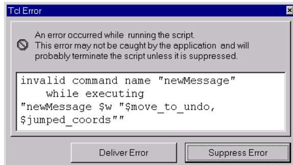
Figure 18 The TclPro Debugger Tcl Error Dialog
