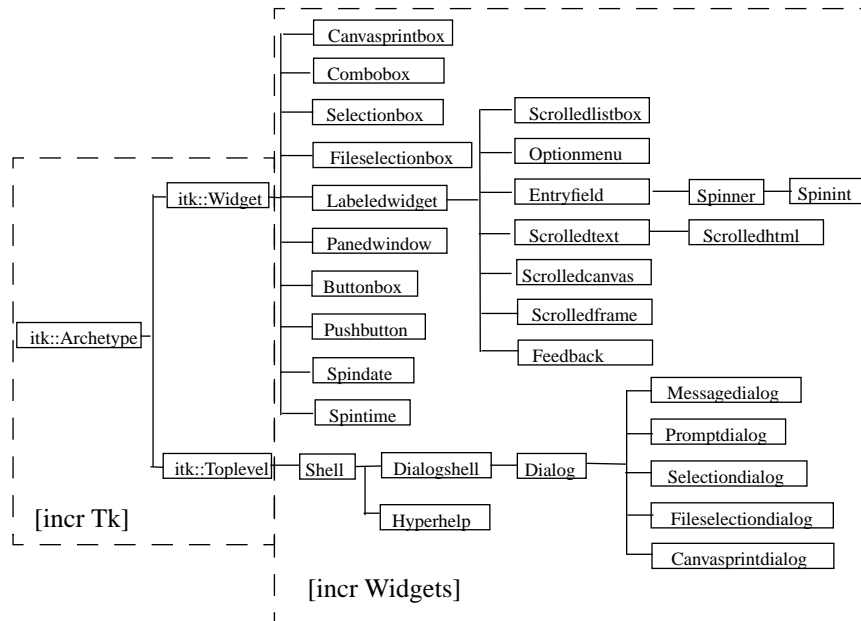
Figure 6-7. [incr Widgets] inheritance hierarchy
