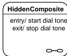
Figure 3-62 Composite State with hidden decomposition indicator icon
