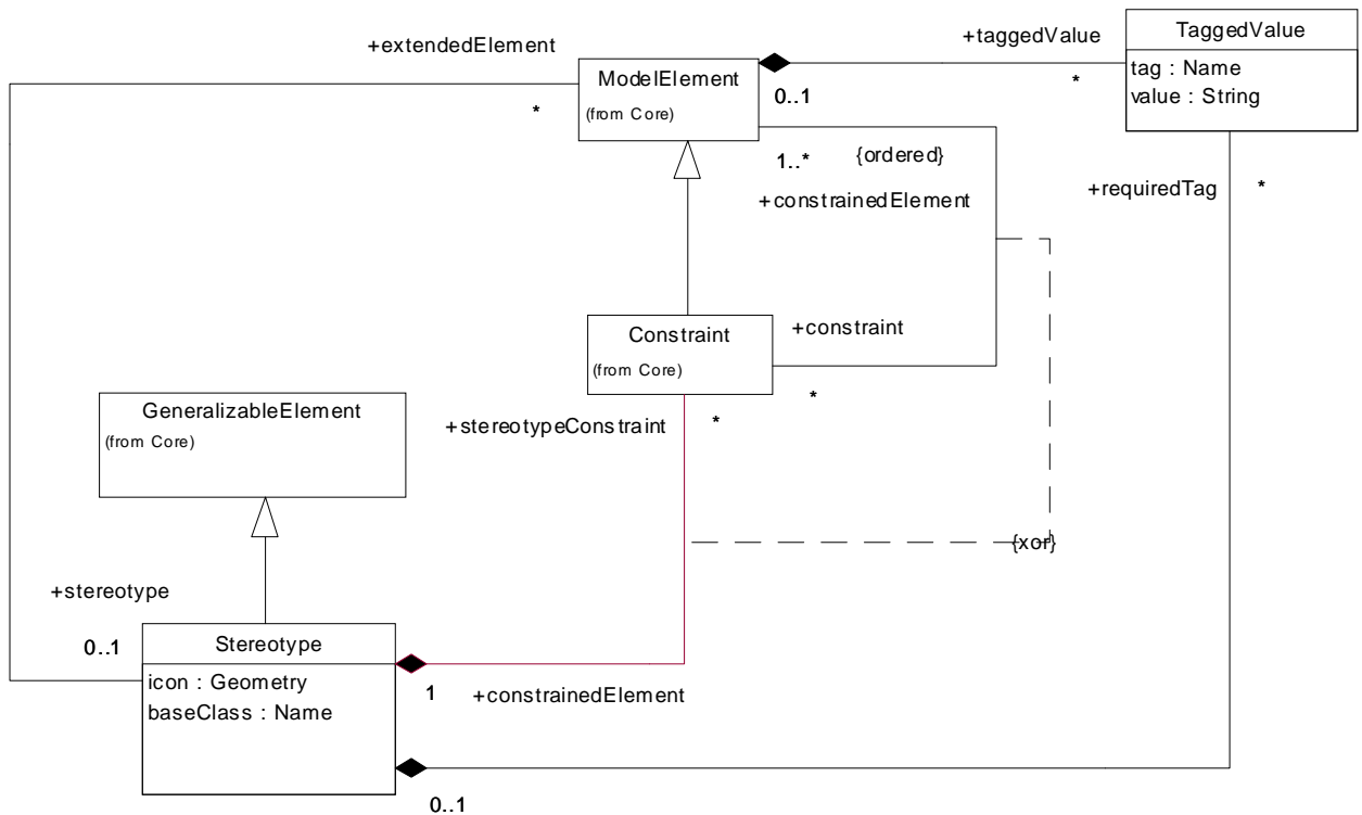
Figure 2-10 Extension Mechanisms
