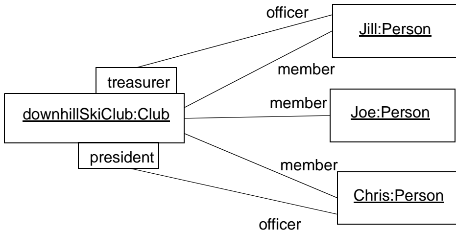
Figure 3-37 Links
