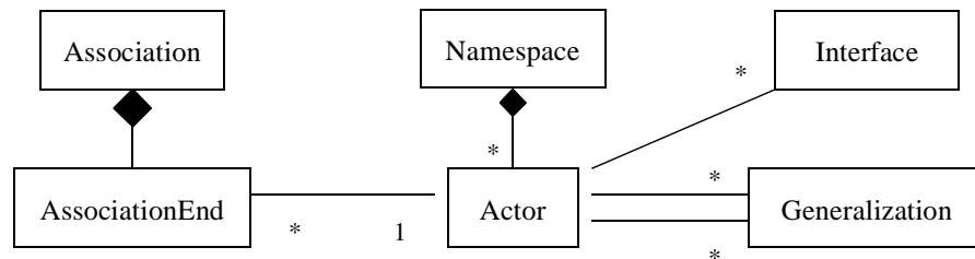
Figure 2-19 Actor Illustration
