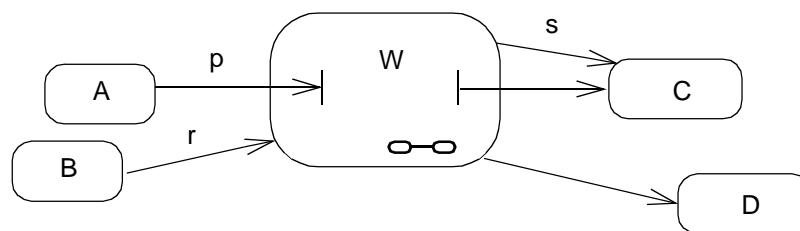
Figure 3-66 Stubbed Transitions
