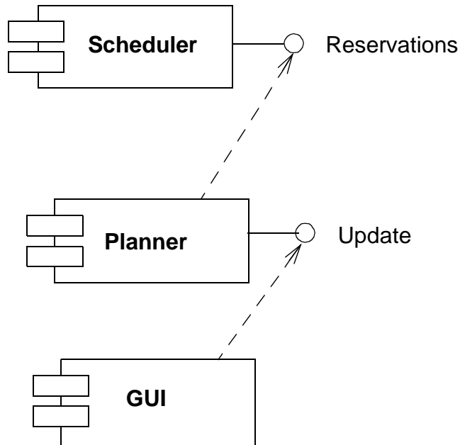
Figure 3-81 Component Diagram
