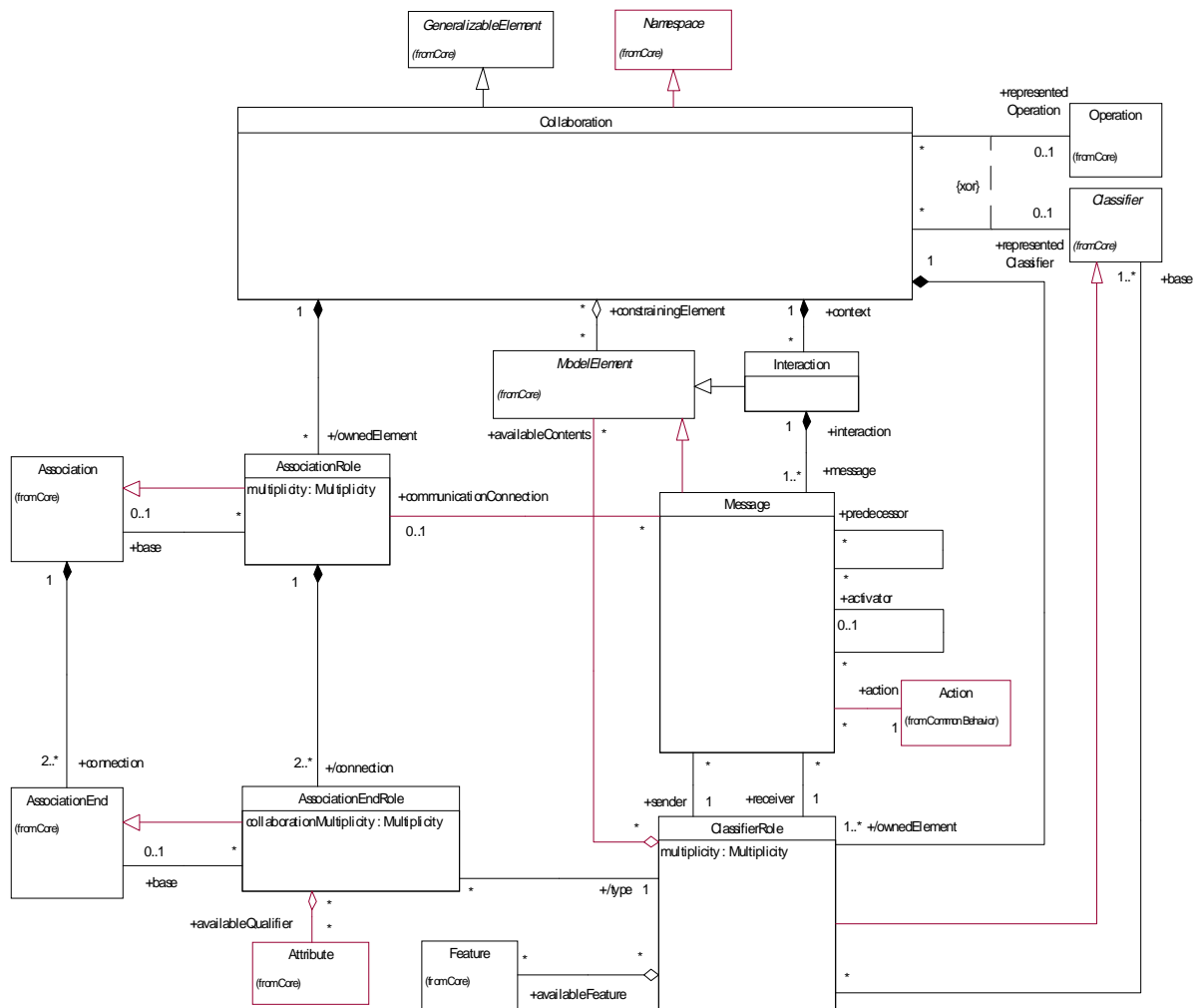
Figure 2-17 Collaborations
