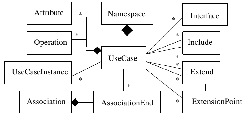
Figure 2-20 UseCase Illustration
