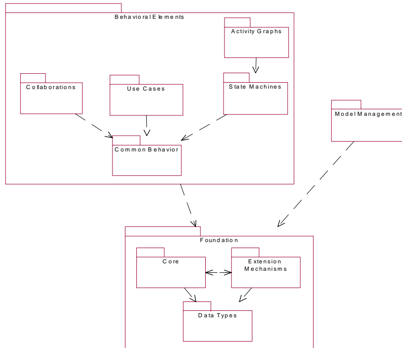
Figure 0-1 UML Class Diagram Showing Package Structure
