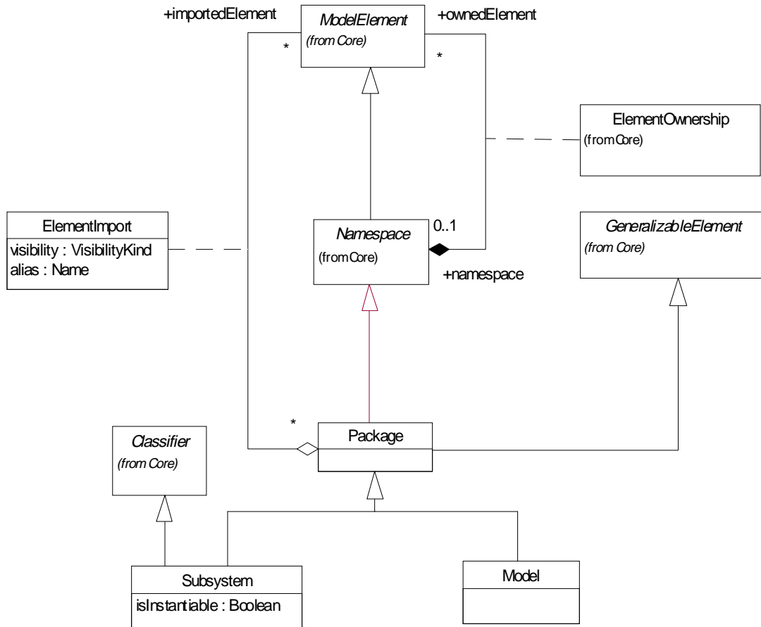
Figure 2-29 Model Management
