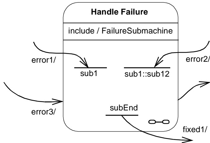
Figure 3-70 Submachine State
