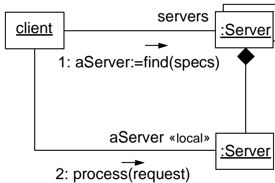
Figure 3-57 Multiobject
