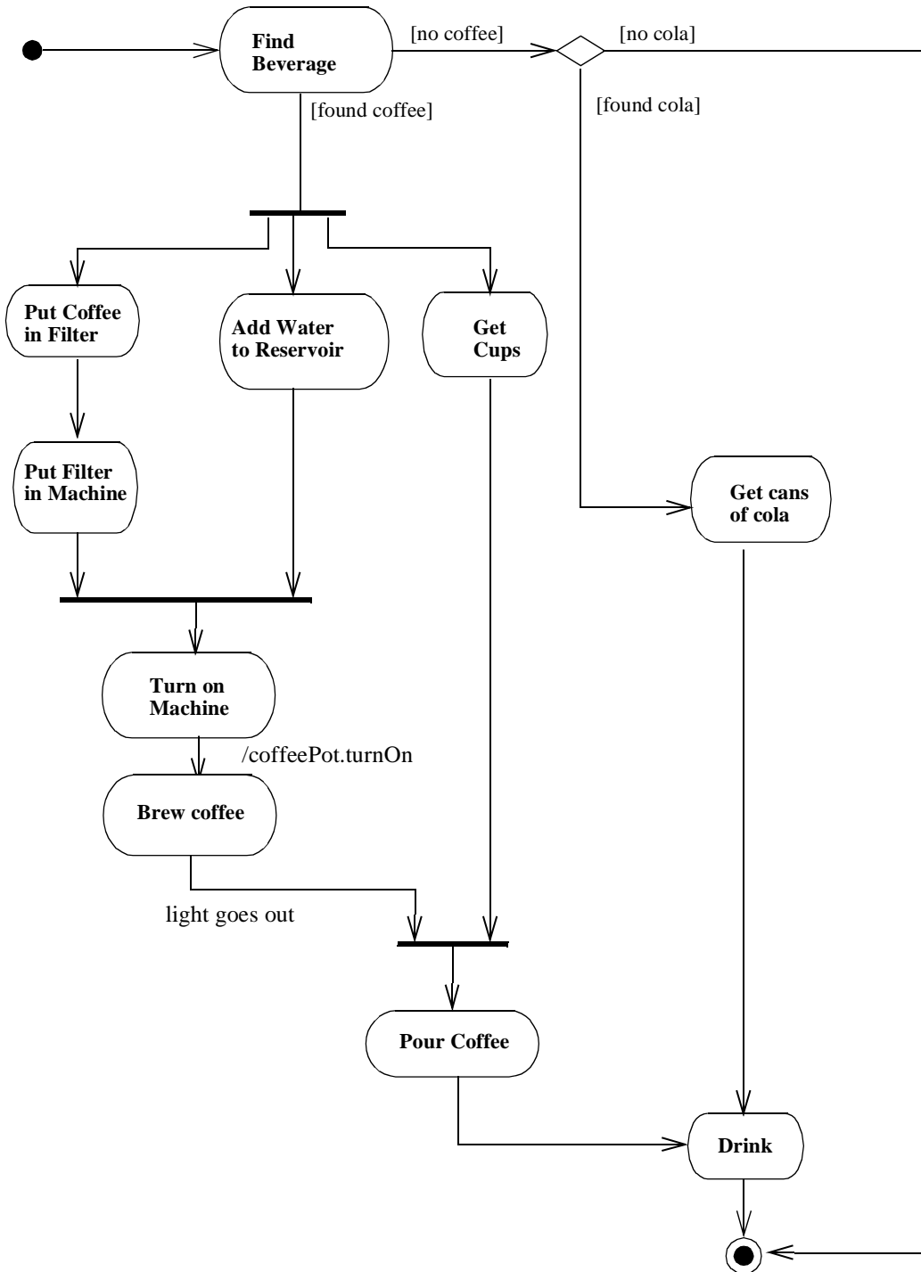
Figure 3-72 Activity Diagram
