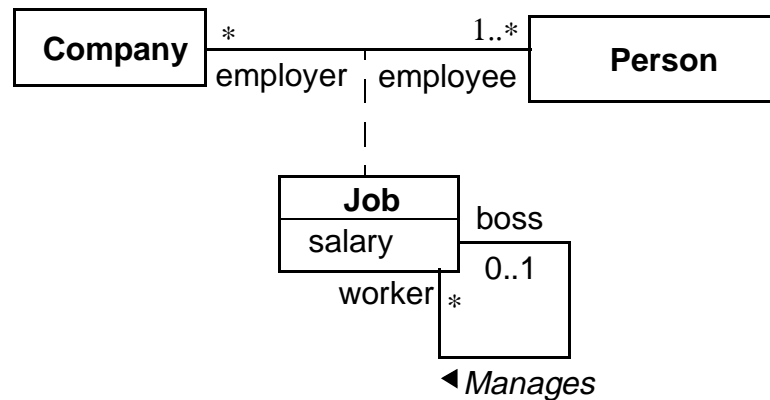
Figure 3-34 Association Class
