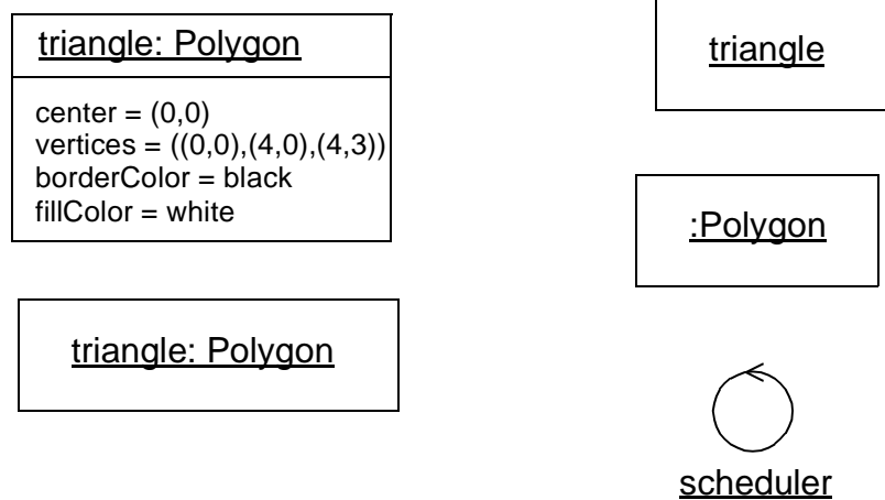
Figure 3-29 Objects
