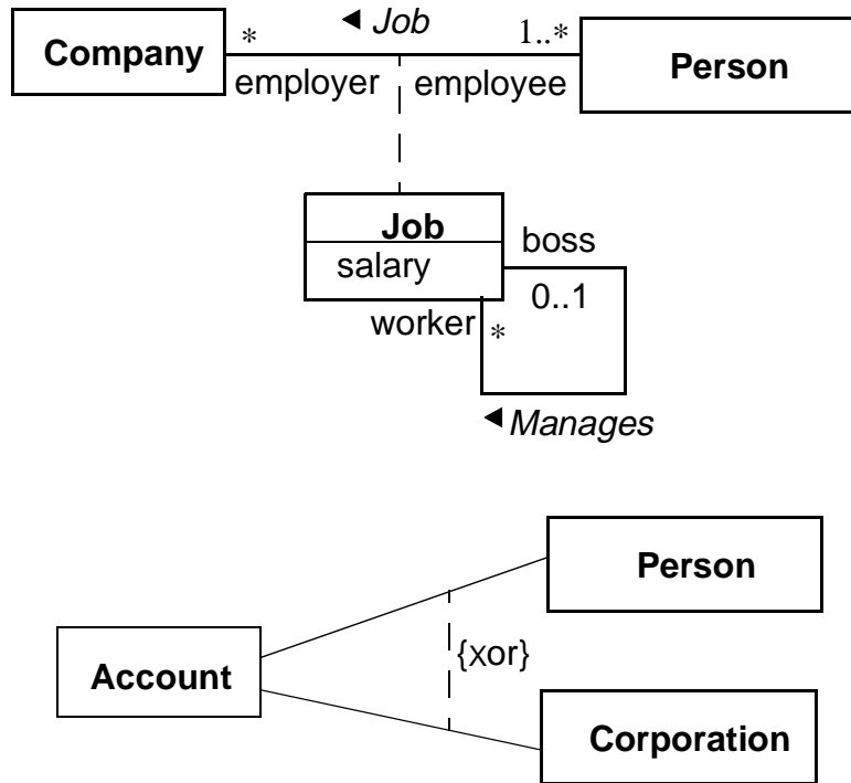
Figure 3-31 Association Notation
