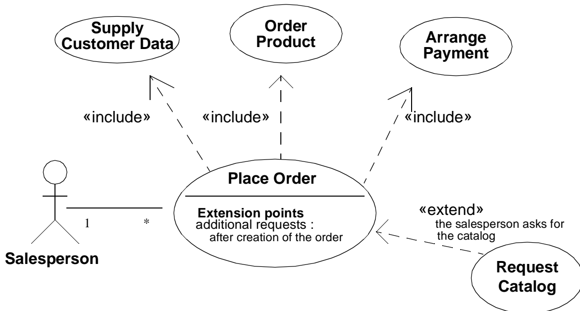
Figure 3-45 Use Case Relationships
