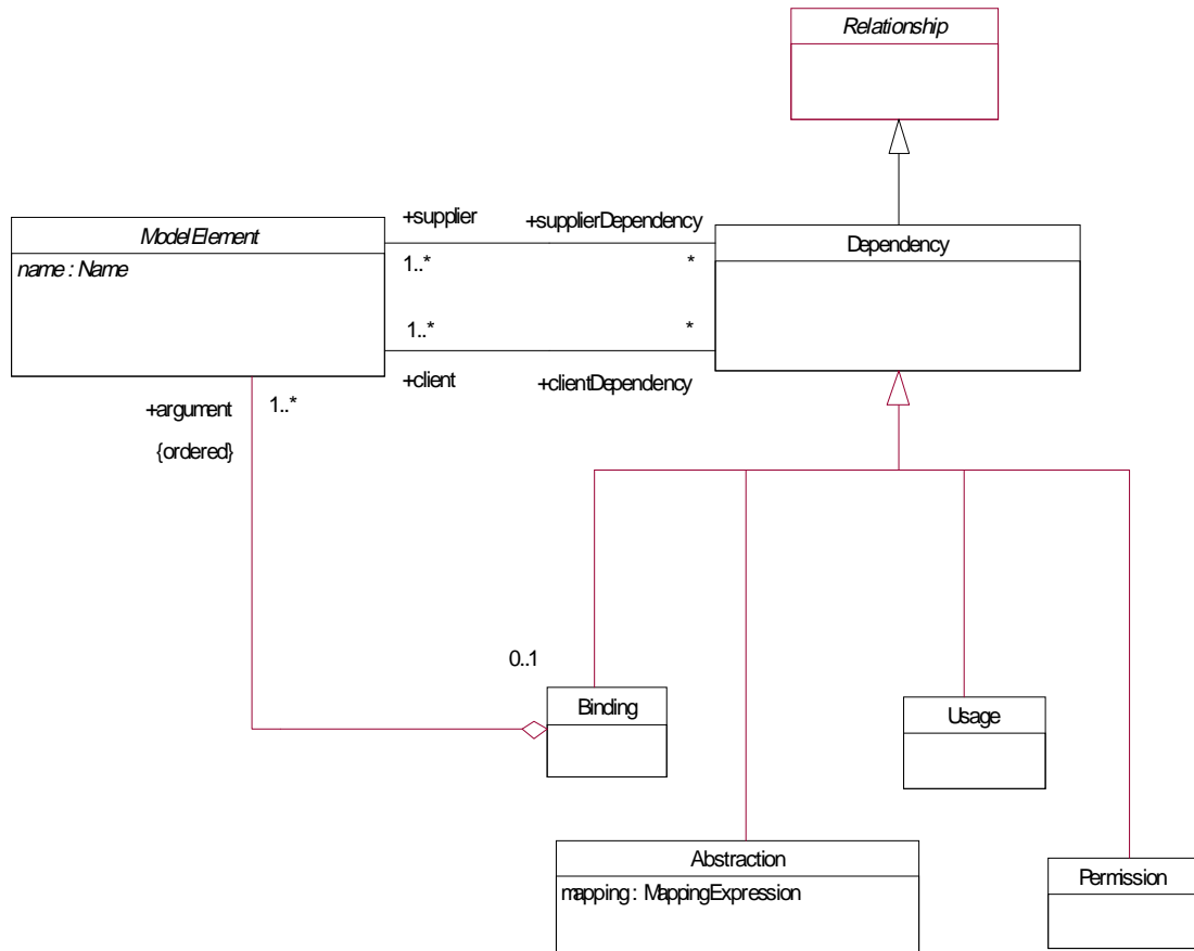
Figure 2-7 Core Package - Dependencies
